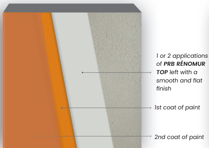
Sound and clean painted substrate (no cracks and flaking)
