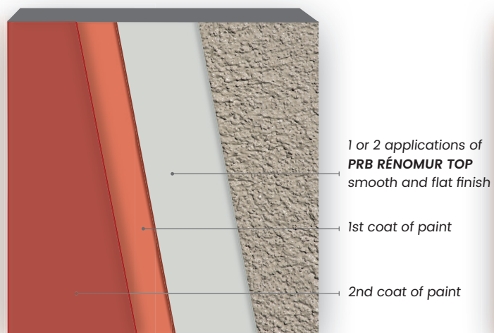
Sound and clean painted substrate (no cracks and flaking)
