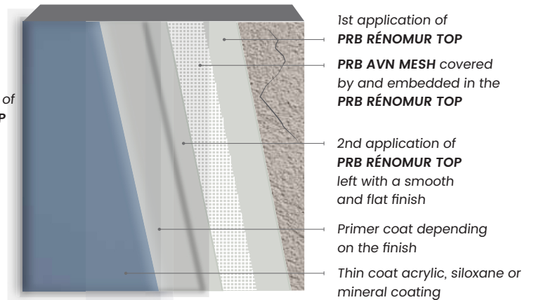
Irregular/uneven, sound and clean painted substrate (crazed and repaired)
