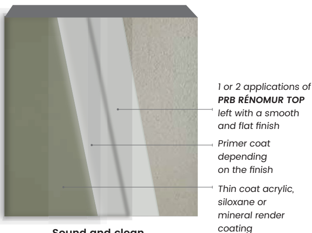
Sound and clean painted substrate (no cracks and flaking)
